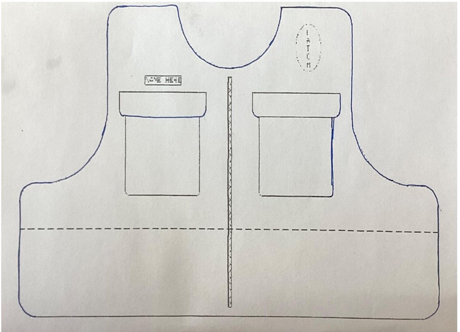
SKETCH PLACEMENT OF OPTIONAL POCKETS ON VEST
